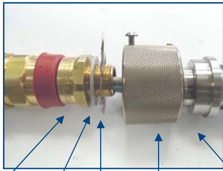
Cable Gland IP Washer Tab Washer Running Coupler Rear Shell
